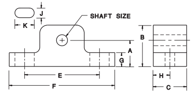
PILLOW BLOCK
